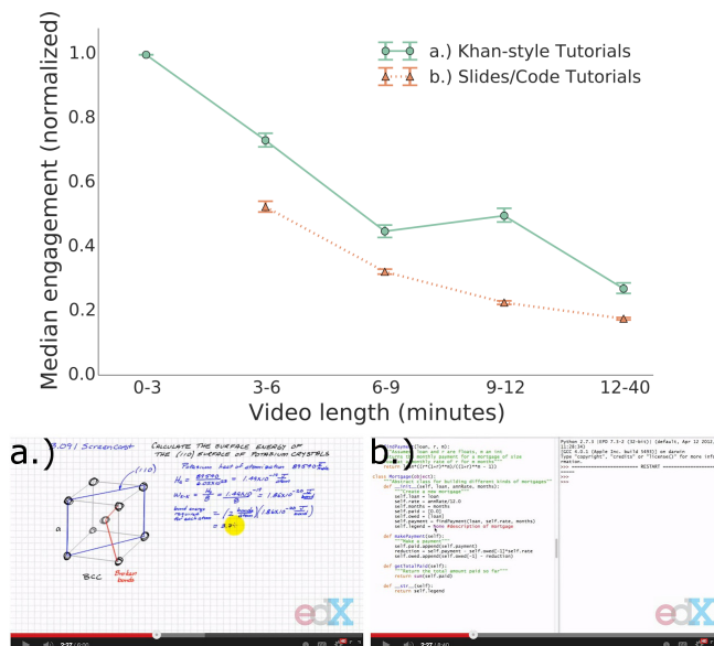
Figure 4. Median normalized engagement times vs. length for tutorial videos. Students engaged more with Khan-style tablet drawing tutorials (a.) than with PowerPoint slide and code screencast tutorials (b.). Error bars are approximate 95% confidence intervals for the true median [14].
